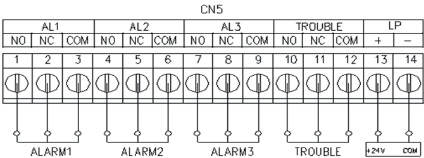
[Figure 6. Relay Terminal Configuration]
