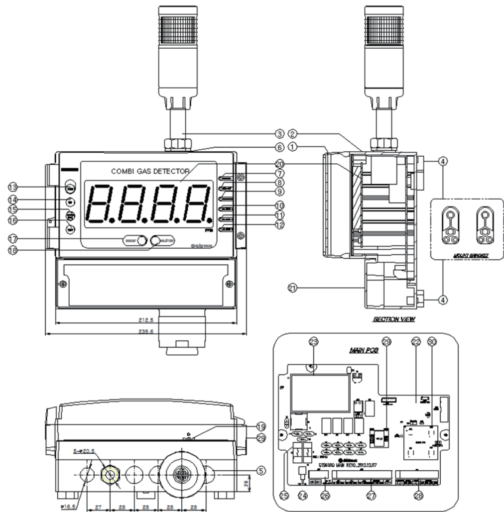
[Figure 2. GTD-6000 Components]
