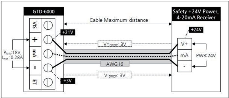
[Figure 8. GTD–6000 Installation Cable Length Calculation]
