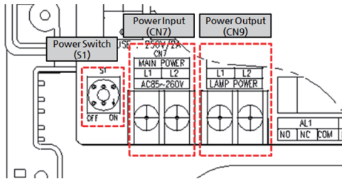
[Figure 4. Power Terminal Configuration]
