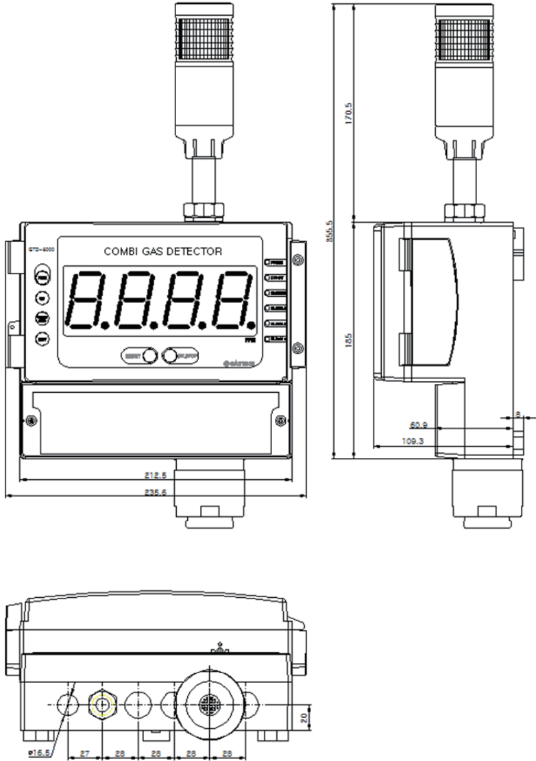
[Figure 9. GTD-6000 Drawing 1]
